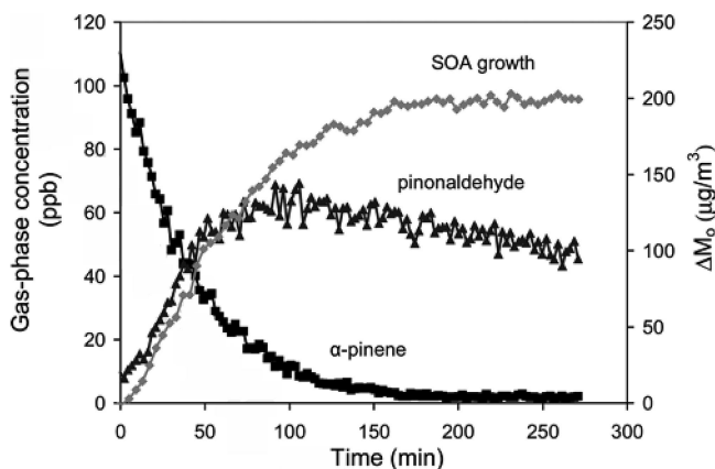
Figure 12. Time evolution of \alpha -pinene and pinaldehyde from \alpha -pinene photo-oxidation as measured by PTR-MS in a reaction-chamber experiment. Also shown is the corresponding secondary organic aerosol (SOA) growth curve, as measured by aerosol mass spectrometry. Reprinted with permission from ref 171. Copyright 2006 American Chemical Society.
